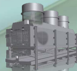
SLKv
